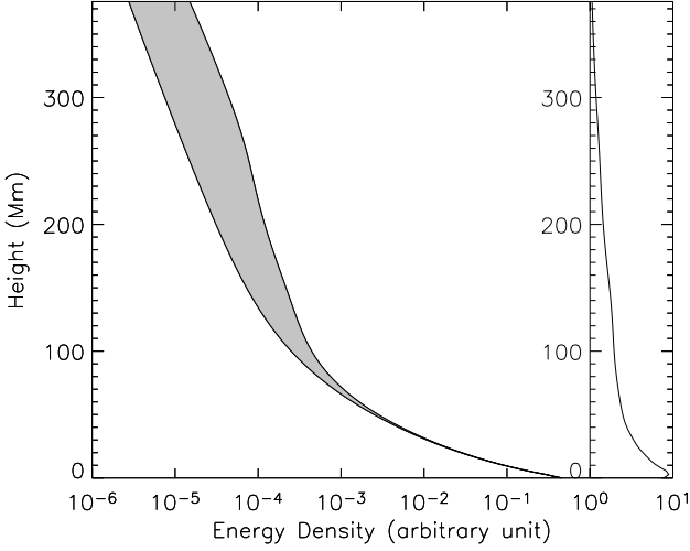
Fig. 10. Variation of the energy density for AR 8210 along the z -axis for the potential field (lower curve) and the nfff field (upper curve) obtained by averaging the magnetic field strength in the corresponding xy -plane. The free magnetic energy is contained in the light gray area. The plot on the right shows the percentage of free energy along the z -axis (see text for details). Note that the energy density axis is measured on a logarithmic scale.
