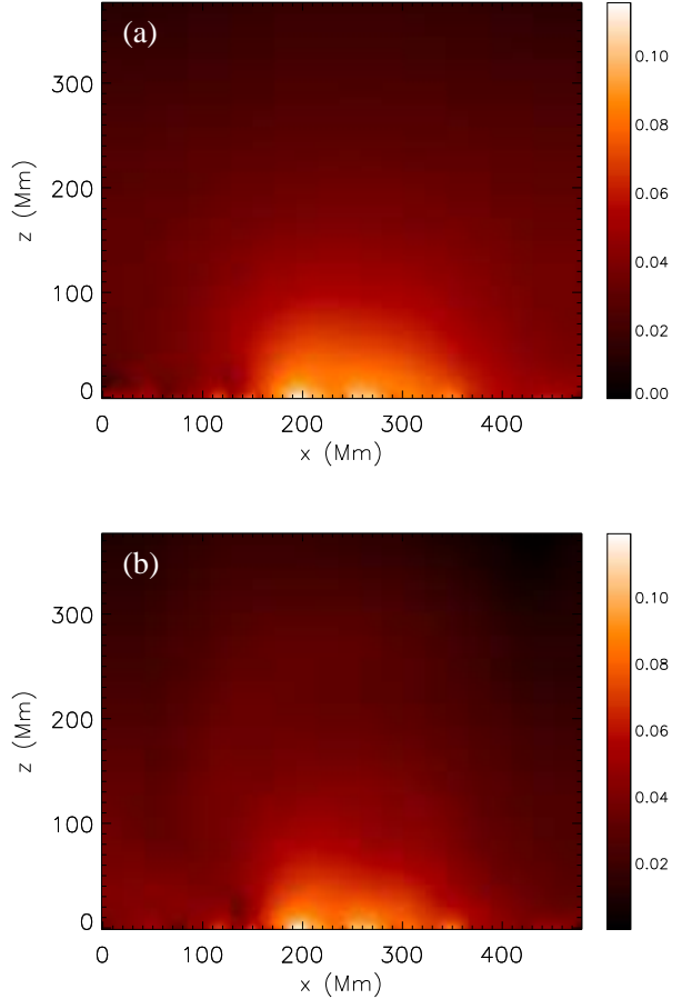
Fig. 9. Energy density maps in the plane y = 60 for AR 8210: (a) potential field, (b) nlff field (increasing density from black to white). The energy density is in arbitrary units and a log scale is used to take into account the rapid decrease of magnetic field strength with height.
