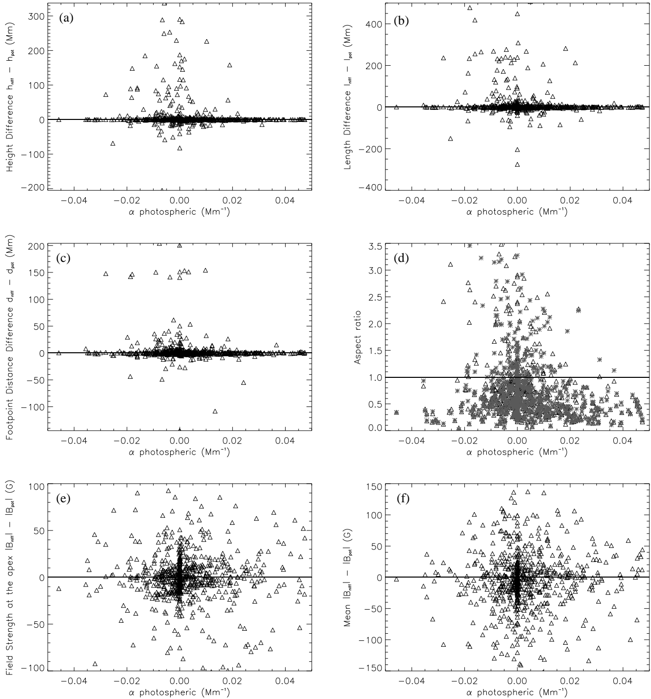
Fig. 6. Differences between the potential and nfff fields for AR 8210. Geometrical parameters: (a) the height, (b) the length and (c) the distance between footpoints as a function of the \alpha value at the footpoint (in units of \text{Mm}^{-1} ). (d) The aspect ratio of each loop is plotted for the nfff (triangles) and for the potential (asterisks). The magnetic field of each loop is characterised by (f) the field strength at the apex and (e) the mean field strength along the loop.
