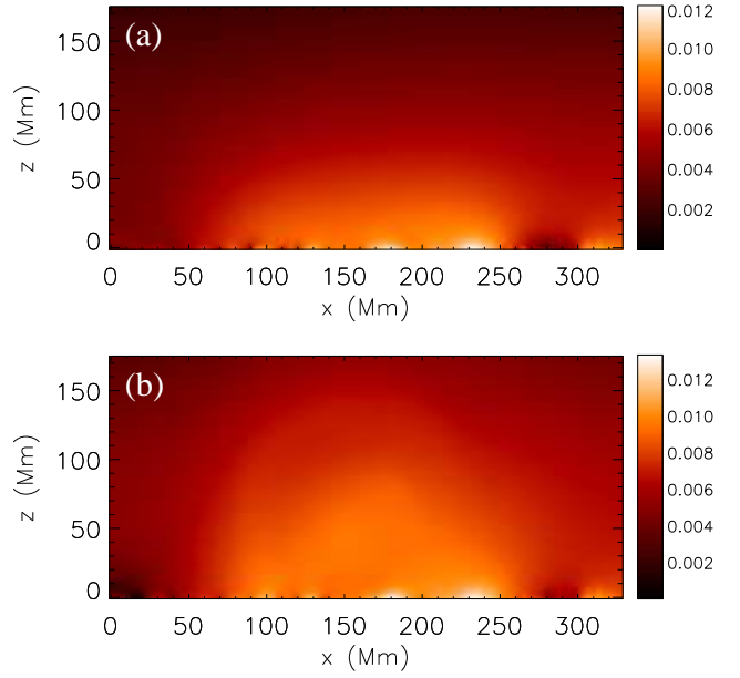
Fig. 7. Energy density maps at y = 60 pixel for AR 8151: (a) potential field, (b) nlff field (increasing density from black to white). The energy density is in arbitrary units and a log scale is used to take into account the rapid decrease of the magnetic field strength with height.
