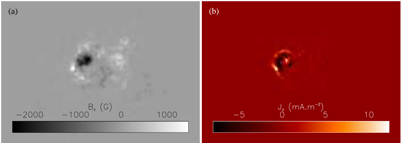
Fig. 2. Photospheric distributions for AR 8210: (a) the vertical component of the magnetic field as observed by IVM; (b) the vertical current density as computed from the transverse components. The IVM field-of-view is surrounded by SOHO/MDI magnetic field for B_z and zero values for J_z (see text for details).
