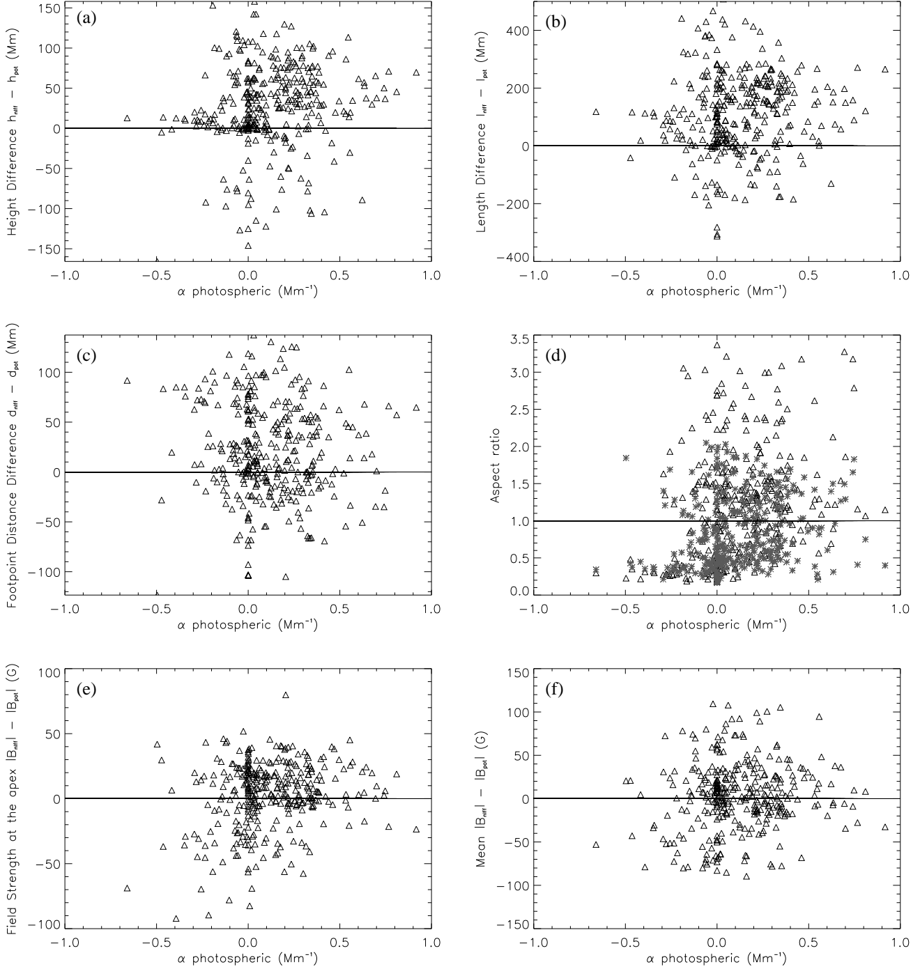
Fig. 5. Differences between the potential and nlff fields for AR 8151. Geometrical parameters: (a) the height, (b) the length and (c) the distance between footpoints as a function of the \alpha value at the footpoint (in units of \text{Mm}^{-1} ). (d) The aspect ratio of each loop is plotted for the nlff (triangles) and for the potential (asterisks). The magnetic field of each loop is characterised by (f) the field strength at the apex and (e) the mean field strength along the loop.
