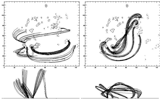
Fig. 3. AR 8151 3D magnetic field configurations for the potential field (left) and for the nlff field (right). A few particular flux bundles are plotted corresponding to the same footpoints in the positive polarity (solid contours). We note that the current density modifies the geometry of the field lines and their connectivity.
