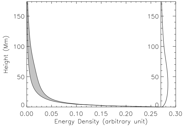
Fig. 8. Variation of the energy density for AR 8151 along the z -axis for the potential field (lower curve) and the nlff field (upper curve) obtained by averaging the magnetic field strength in the corresponding xy -plane. The free magnetic energy is contained in the light gray area. The plot on the right shows the percentage of free energy along the z -axis (see text for details).
