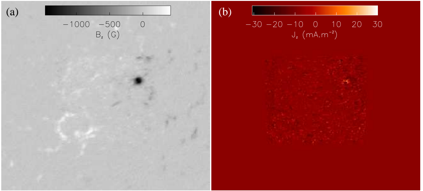
Fig. 1. Photospheric distributions for AR 8151: (a) the vertical component of the magnetic field as observed by IVM; (b) the vertical current density as computed from the transverse components. The IVM field-of-view is surrounded by SOHO/MDI magnetic field for B_z and zero values for J_z (see text for details). The observations were recorded on February 11, 1998 at 17:36 UT in a composite field-of-view (SOHO/MDI and IVM) of 330'' \times 300'' .
